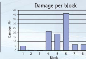
Damage at the critical location from each road surface
