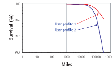
Estimated 'warranty curve' for two user profiles, combines material variability and load variability
