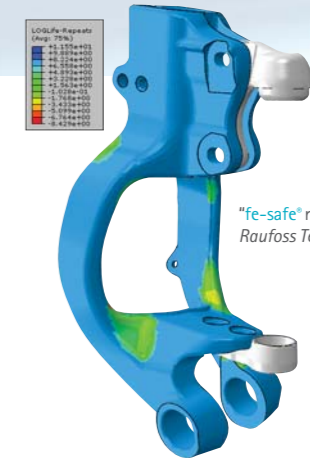
fe-safe® fatigue life contour plot
