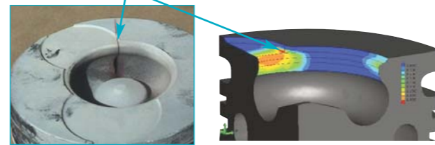
fe-safe® fatigue life contour plot
