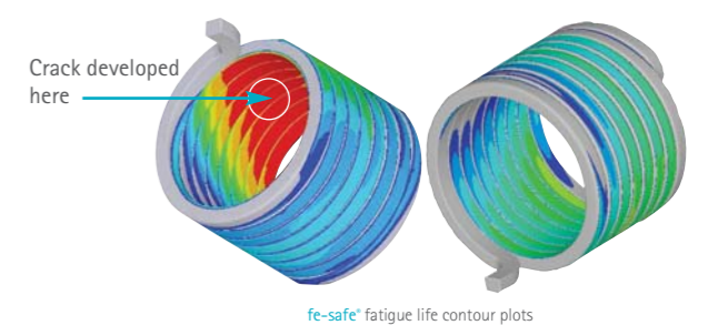
fe-safe fatigue life contour plots
